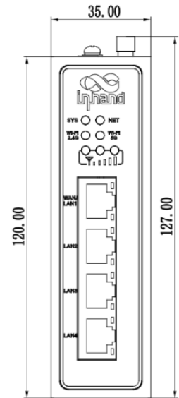
Interface Diagram
